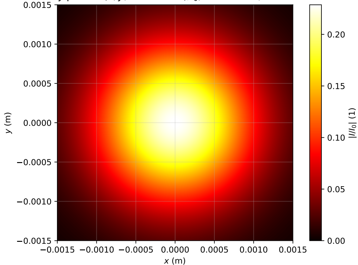
Intensity profile I(x, y, z = 3.901m)/I_0 , P_{in}=0.1P_{cr} , artificial time
